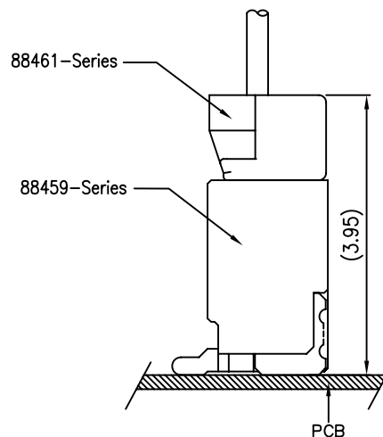
MATE DRAWING
