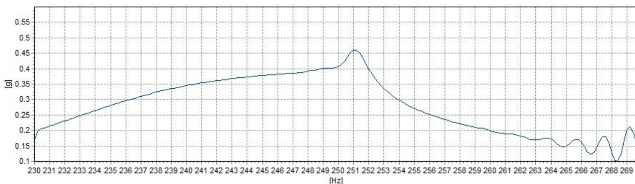
Figure 1: Linear Vibrator Frequency Characteristics/频率特性
