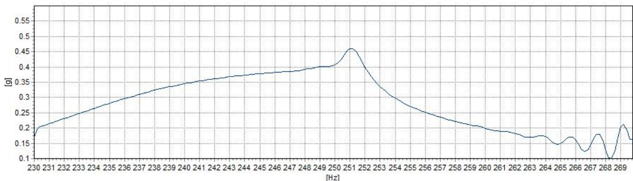
Figure 1: Linear Vibrator Frequency Characteristics/频率特性
